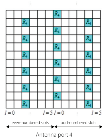
Figure 9. MBMS-SFM reference signal
