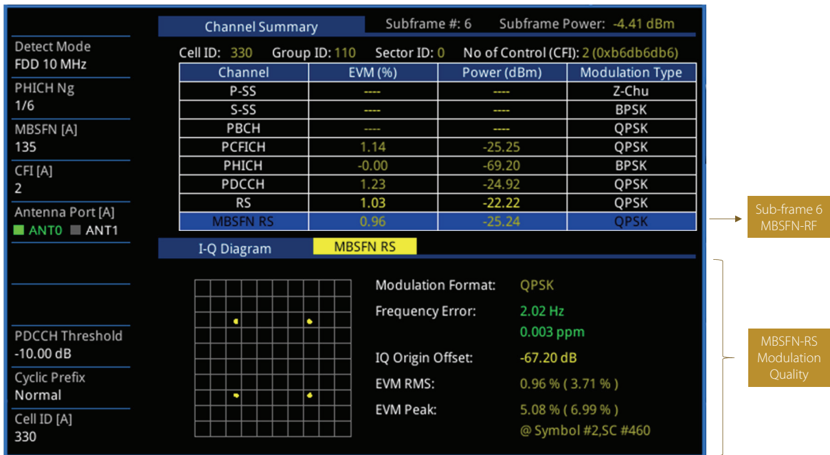
Figure 10. CellAdvisor MBMB SFN reference signal (MBSFN RS)
