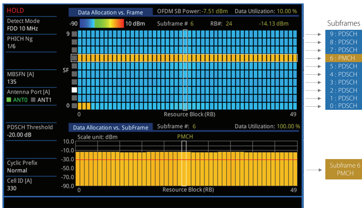
Figure 6. CellAdvisor™ LTE frame analysis — unicast (PDSHC) and broadcast (MBMS) allocations
